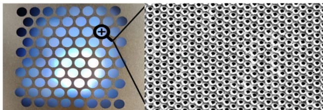
Image 2: In the microplastic filter, the films with the microholes are fixed on a coarser grid so that they do not tear under the water pressure. © Fraunhofer ILT, Aachen, Germany.
