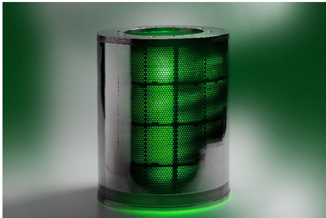
Image 1: 59 million holes in the filter plate of the first laser-drilled filter for the filtration of microplastics from municipal wastewater. © Fraunhofer ILT, Aachen, Germany.
